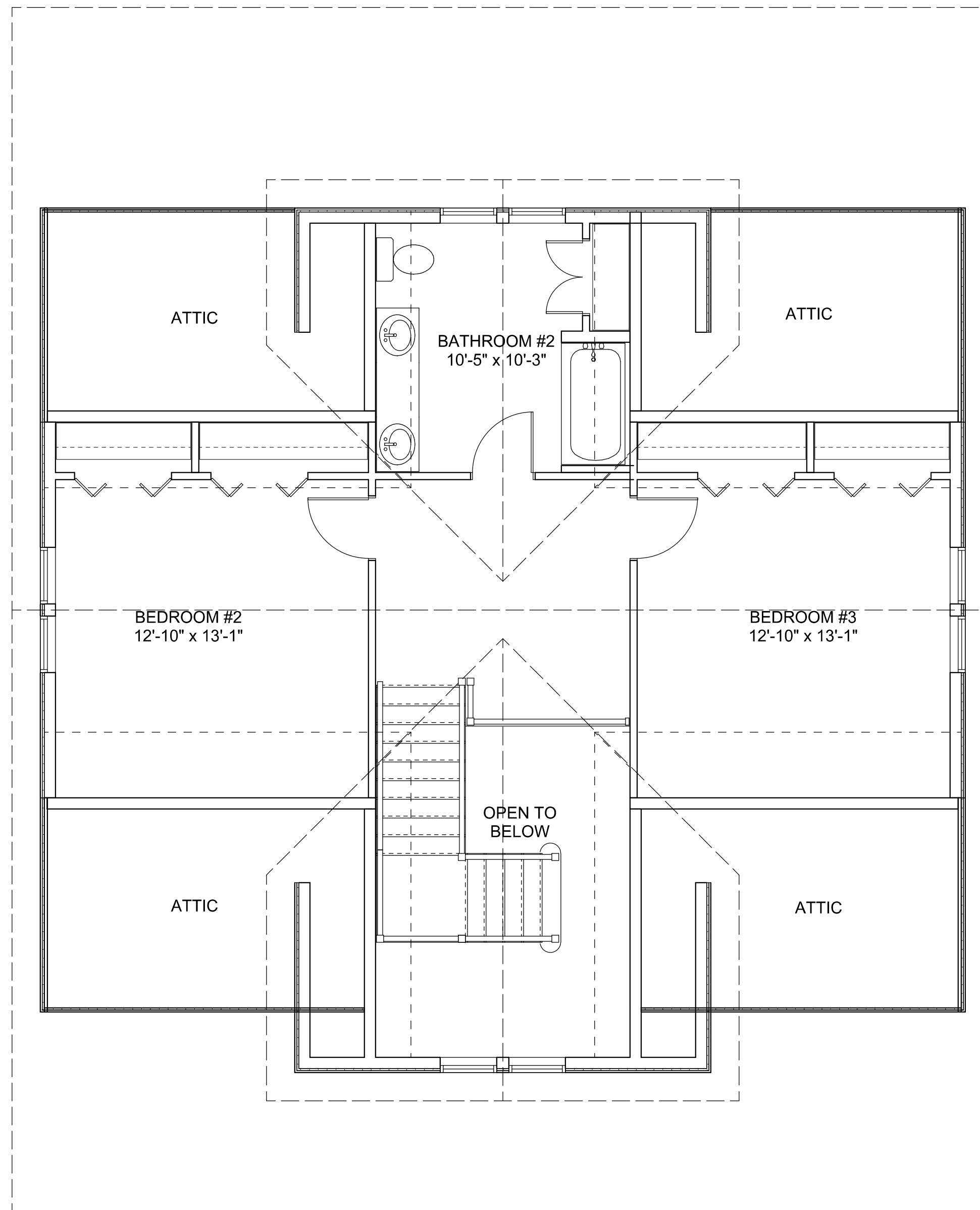
The Lleyton Second Floor Plan
