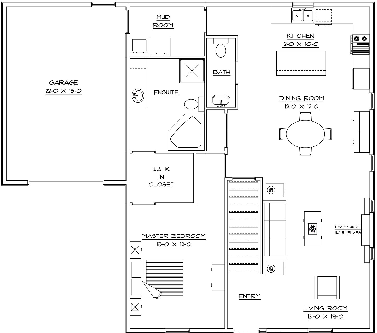
THE CARLIN MAIN FLOOR PLAN 1219 SF
